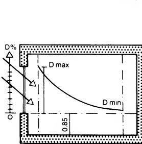
④3 Uniformity; light from the side
